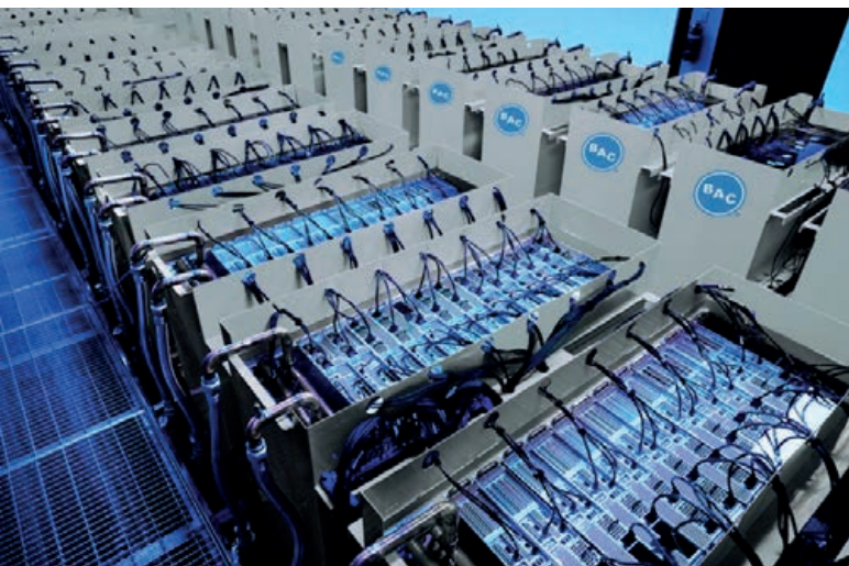
BAC's immersion cooling tanks with CorTex technology. Photo credit: BAC.
