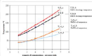
Figure 3: Discharge and oil temperatures for Design of Experiment A and B
