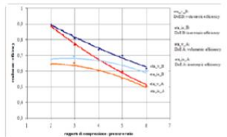
Figure 4: Volumetric and Isentropic efficiencies for Design of Experiments A and B
