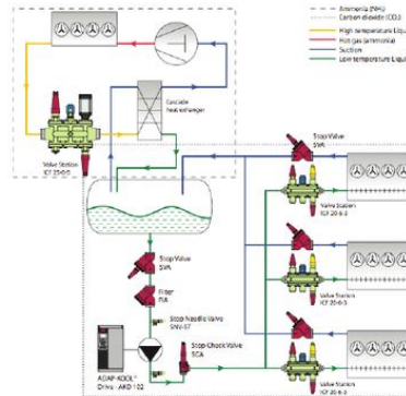
figure 4: overview of controls and valves used in a system using \text{CO}_2 as a secondary refrigerant source: Danfoss
