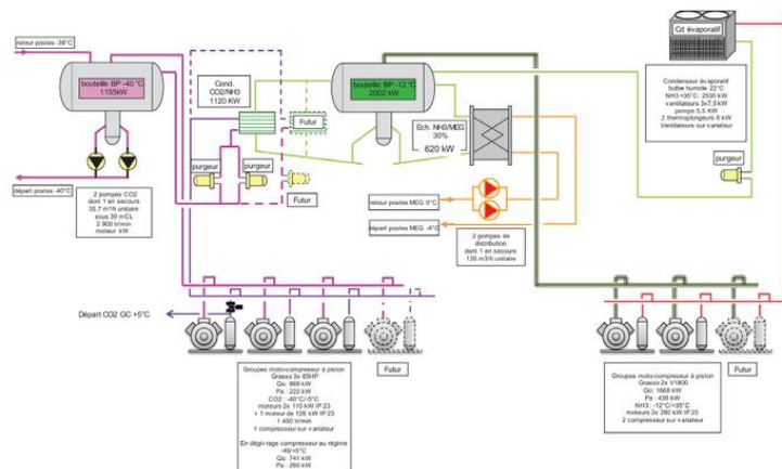
figure 7: Schematic diagram of the refrigeration plant at Lubrano et Fils, in Sète, France
